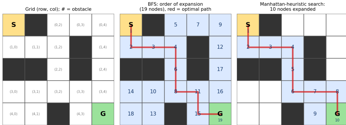
Fig. 2: Grid, BFS expansion order (19 nodes) and Manhattan-heuristic expansion order (10 nodes)
