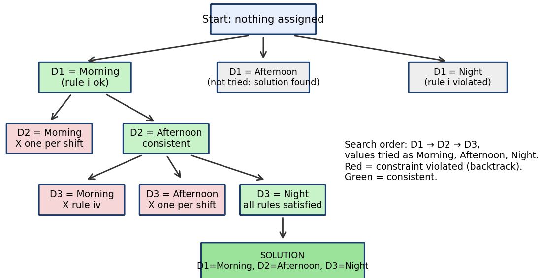
Fig. 1: Backtracking search tree for the doctor-shift problem
